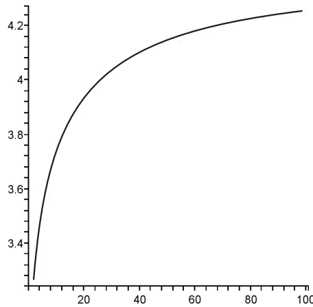
Figure 4. The graph \frac{\ln(T(n)/2)}{\ln(n+1)} , 1 \leq n \leq 100 .
