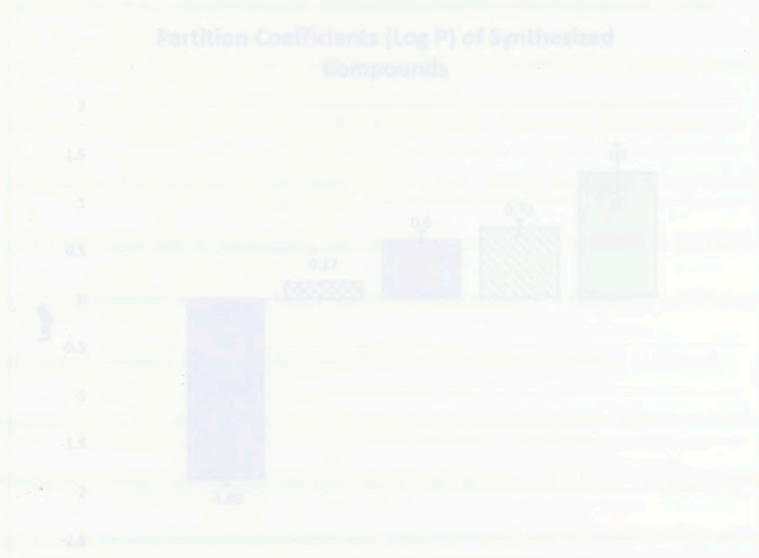
Figure 4. Partition Coefficient of Synthesized Compounds. Compound identification: Compound 1 (Dark blue), Compound 2 (Crosshatched), Compound 3 (Medium blue), Compound 4 (Diagonal lines), and Compound 5 (Light blue with dark outline). The octanol/water coefficient of compounds 1-5 was determined in a microscale assay. Positive Log P values represent an increased affinity for the octanol layer.
