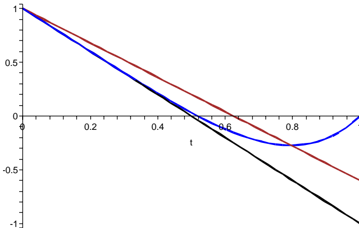
Figure 2: The graph of \psi
