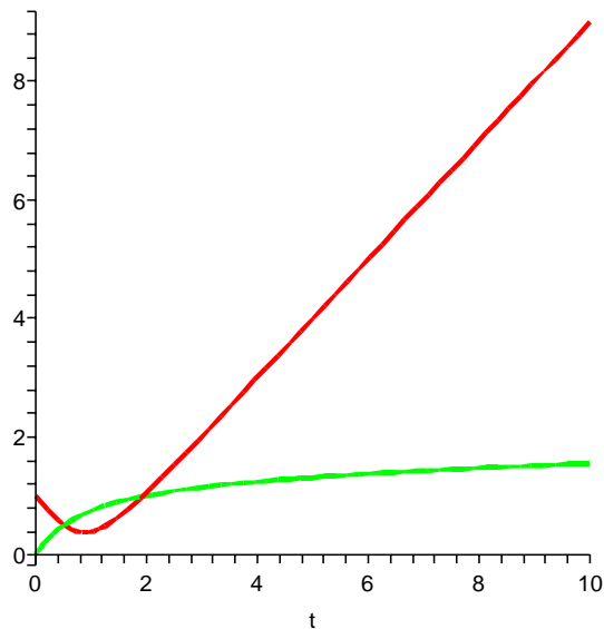
Figure 3: The graphs of \gamma_1, \gamma_2
