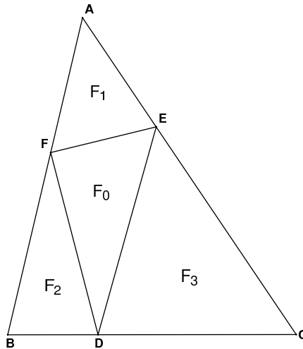
Figure 1: Triangle \triangle ABC
